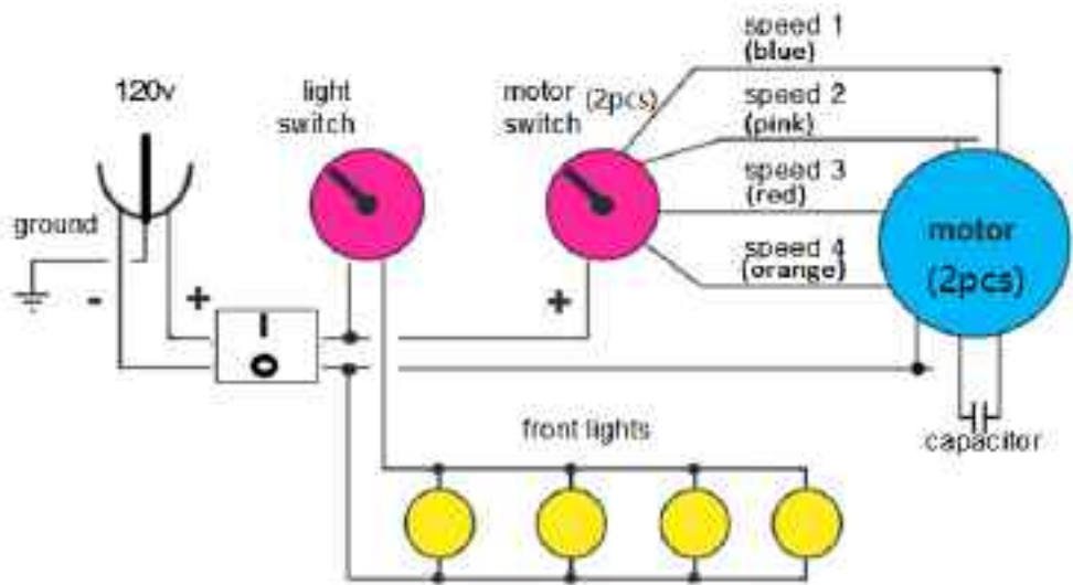
Wiring Diagram
